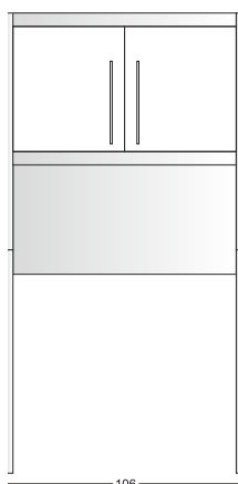
SLD 100 - H2060
