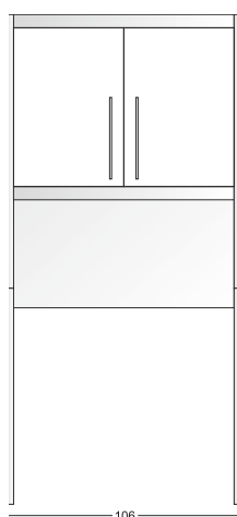
SLD 100 - H2220
