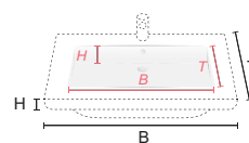
MWCOSR12 120,4 x 2,0 x 41,5/49,5,0 cm B x H x T 59,1 x 12,0 x 33,7 cm
